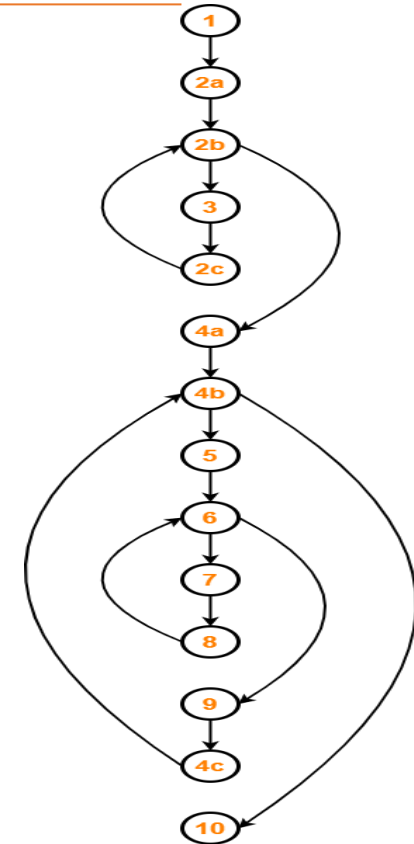
Control Flow Graph
