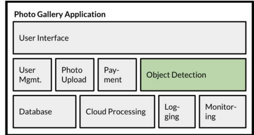
ML System
