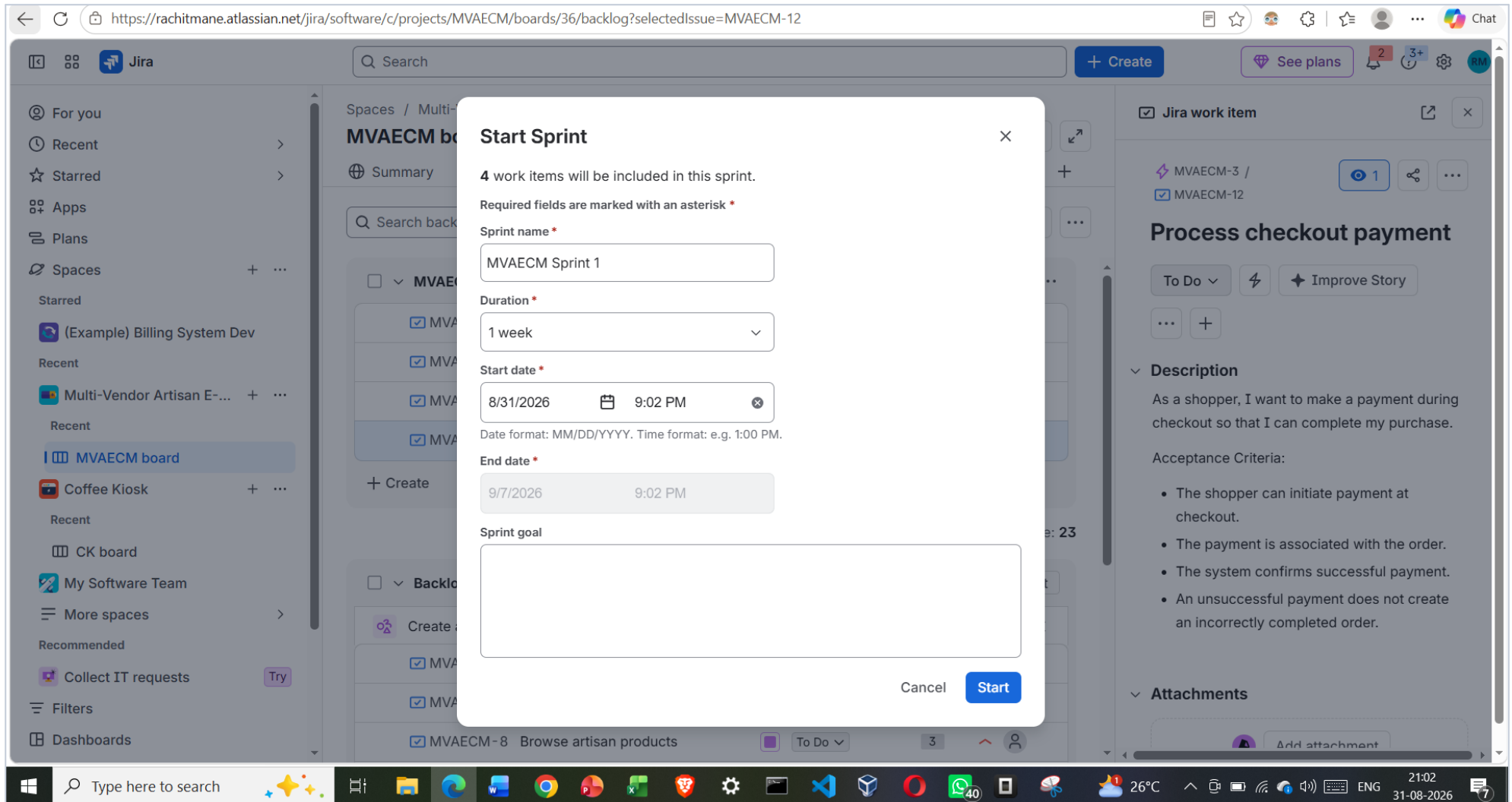
Figure 5 - Creating and starting MVAECM Sprint 1: sprint name "MVAECM Sprint 1", duration 1 week, start date 31/08/2026 9:02 PM, end date 07/09/2026 9:02 PM, with 4 work items included in the sprint.
