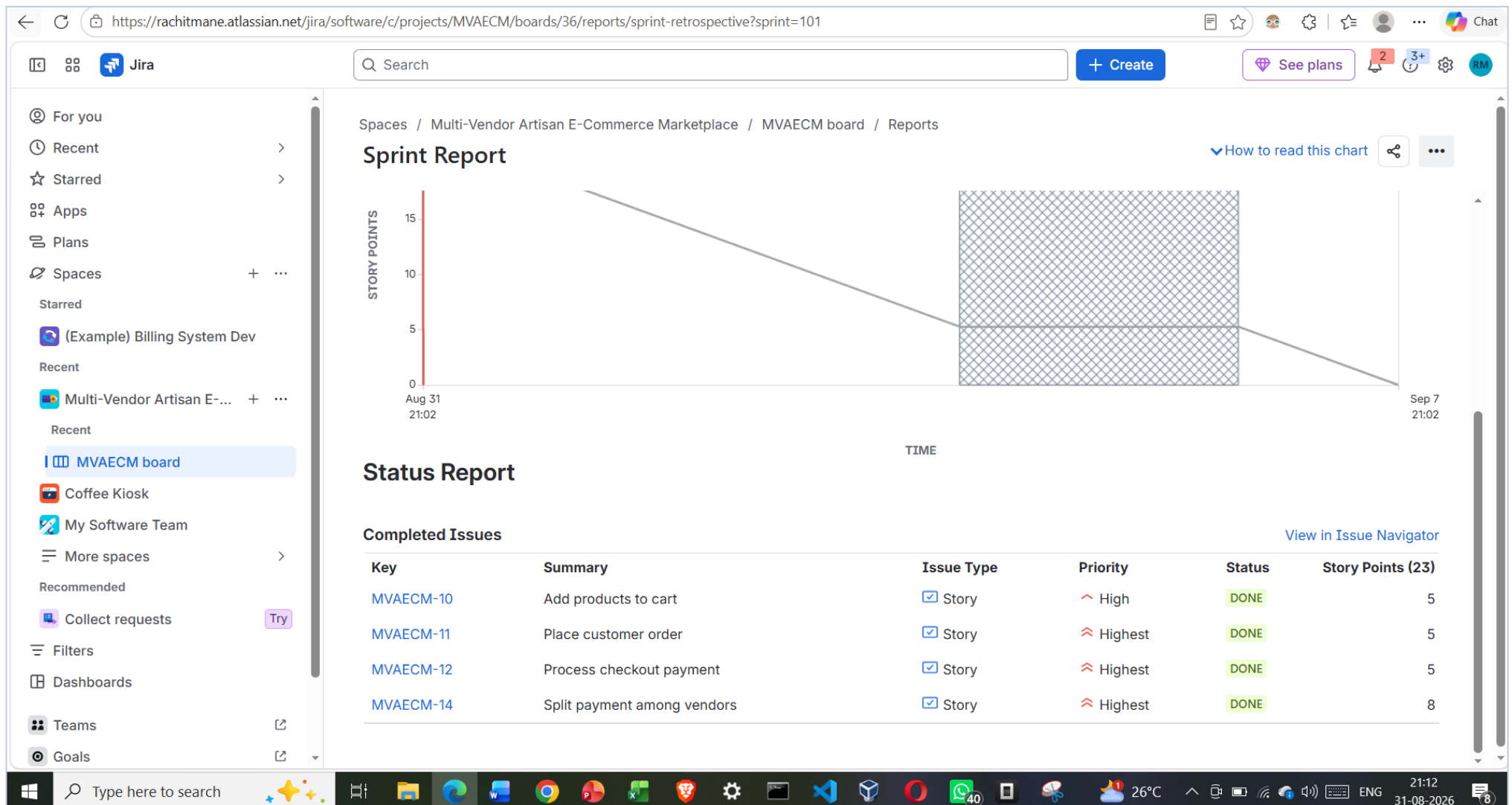
Figure 16 - Sprint Report status report - completed issues: MVAECM-10 Add products to cart (High, 5), MVAECM-11 Place customer order (Highest, 5), MVAECM-12 Process checkout payment (Highest, 5) and MVAECM-14 Split payment among vendors (Highest, 8). Total 23 story points.
