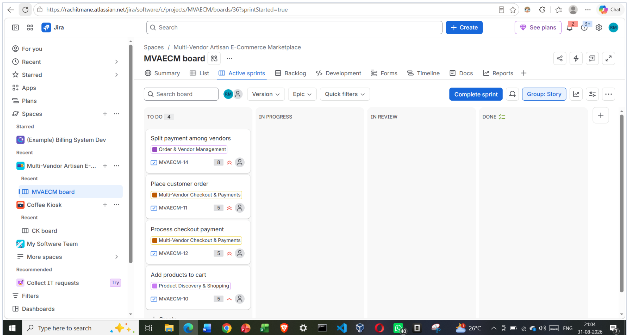
Figure 6 - MVAECM Sprint 1 started. The active sprint board shows the four committed stories in the TO DO column: MVAECM-14 Split payment among vendors (8), MVAECM-11 Place customer order (5), MVAECM-12 Process checkout payment (5) and MVAECM-10 Add products to cart (5).
