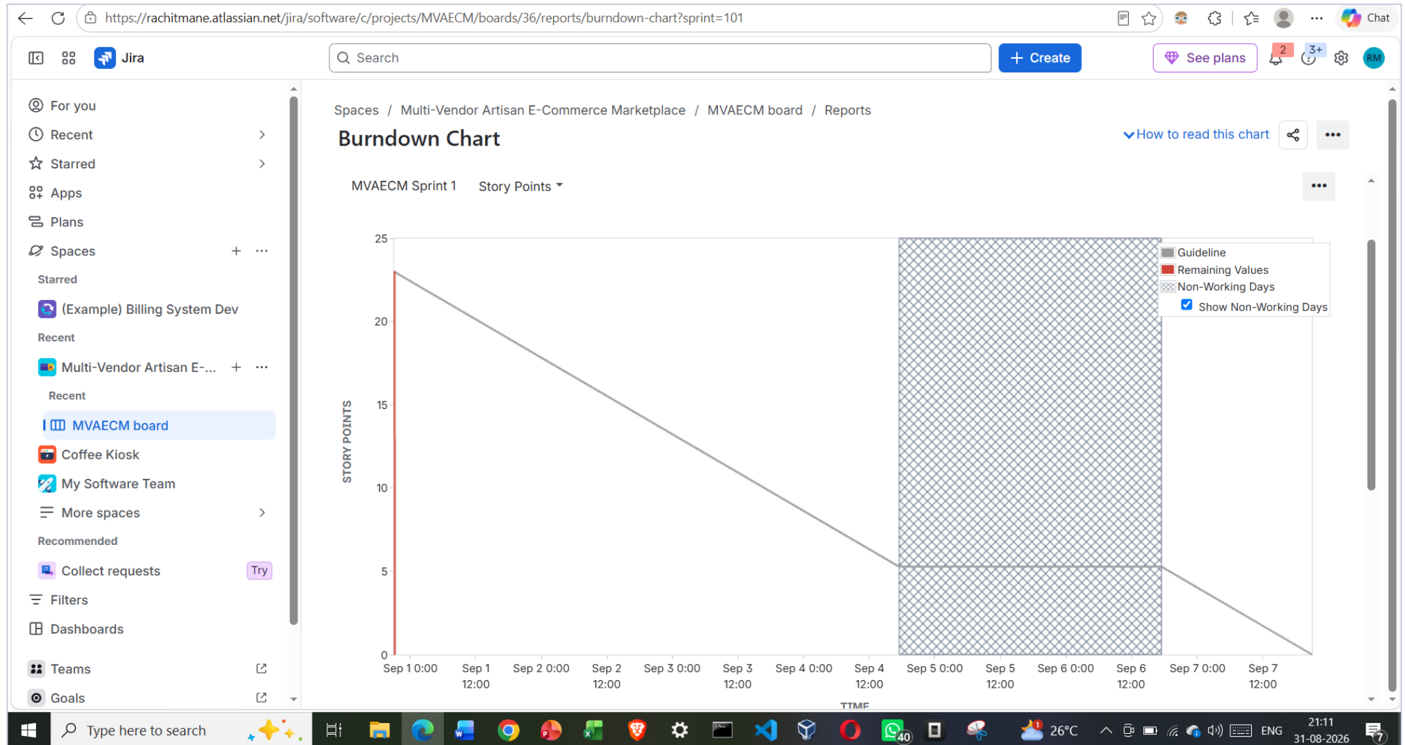
Figure 19 - Burndown chart for MVAECM Sprint 1, measured in story points, starting from the 23 story points committed to the sprint.
