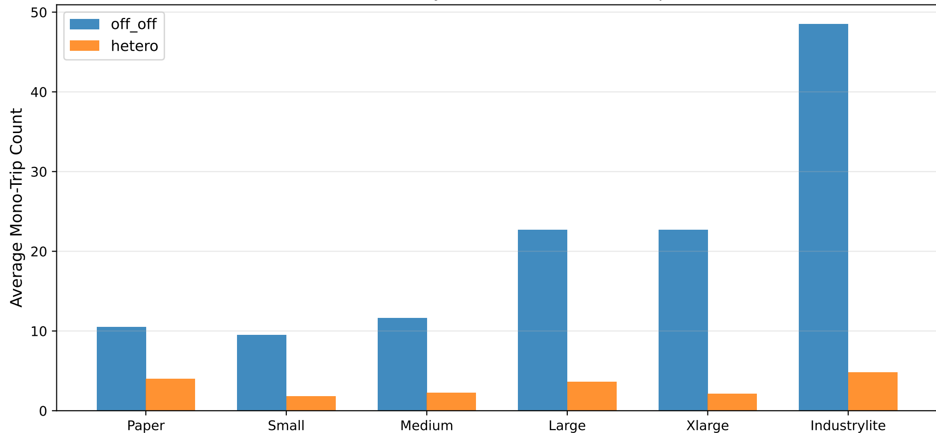
Hetero Penalty Eliminates Mono-Part Trips
