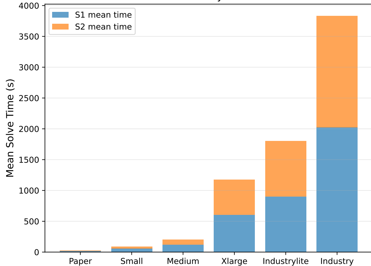
Total Solve Time by Instance Size
