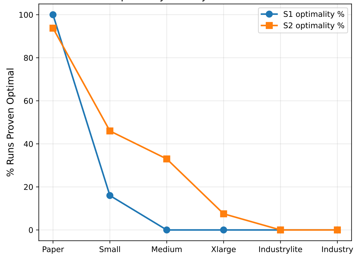
Optimality Rate by Instance Size
