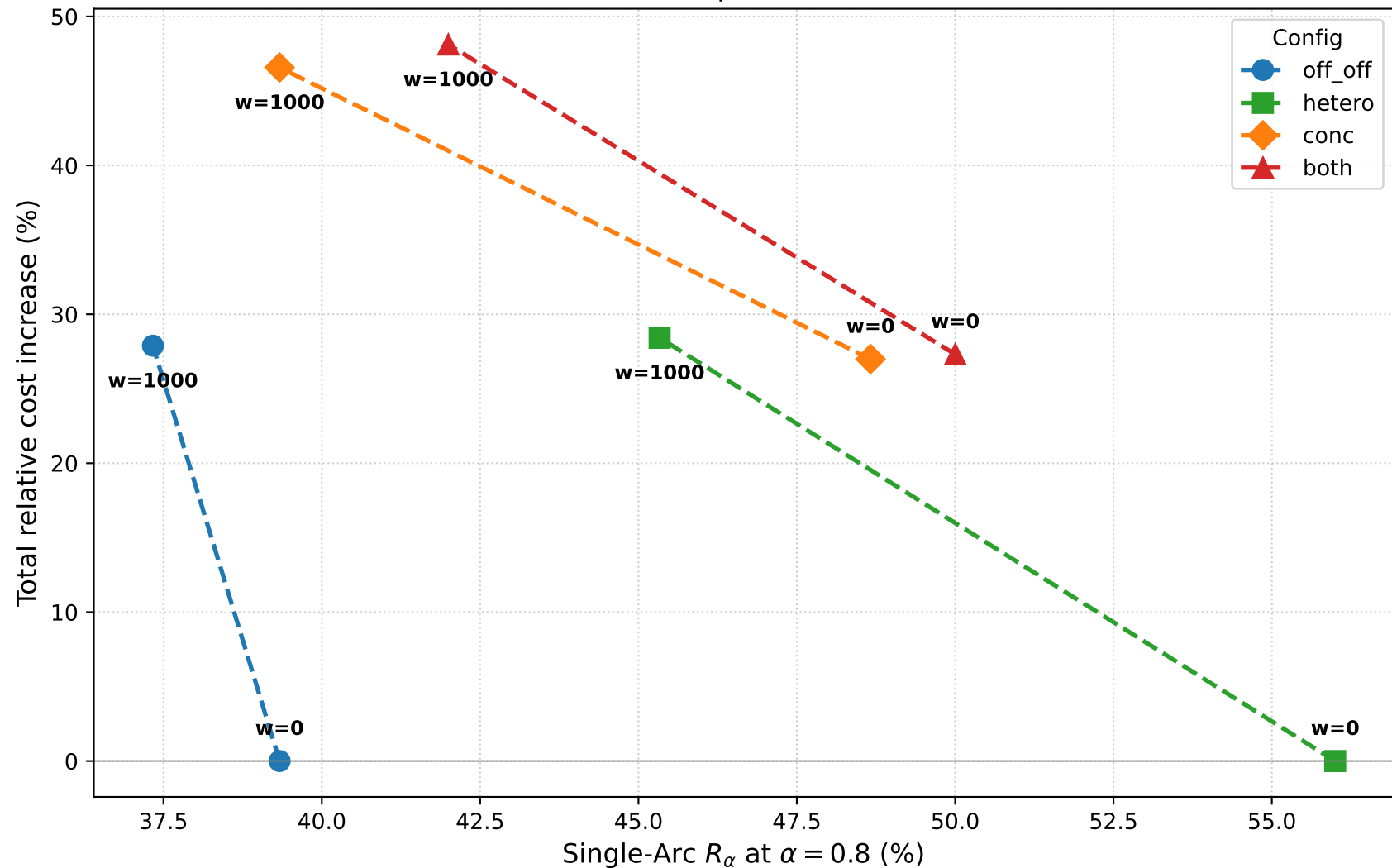
Total costs vs Disruption Tolerance (Small)
