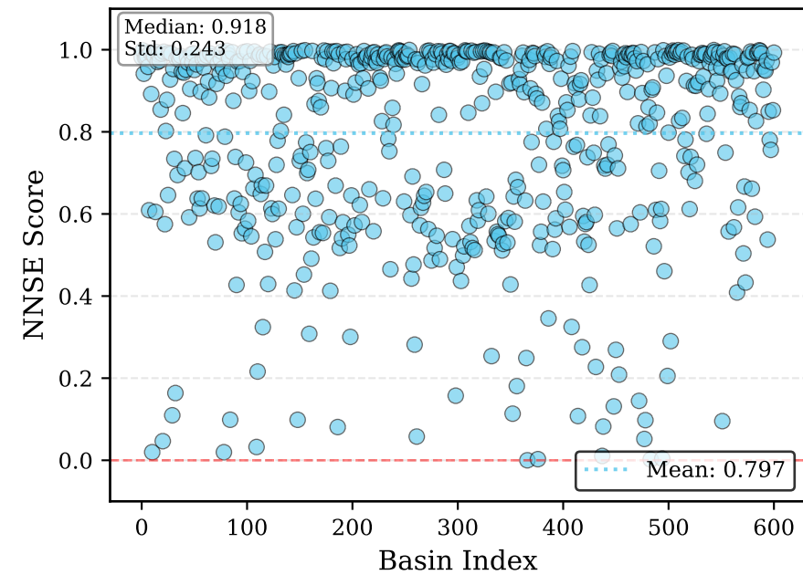
FEDformer
