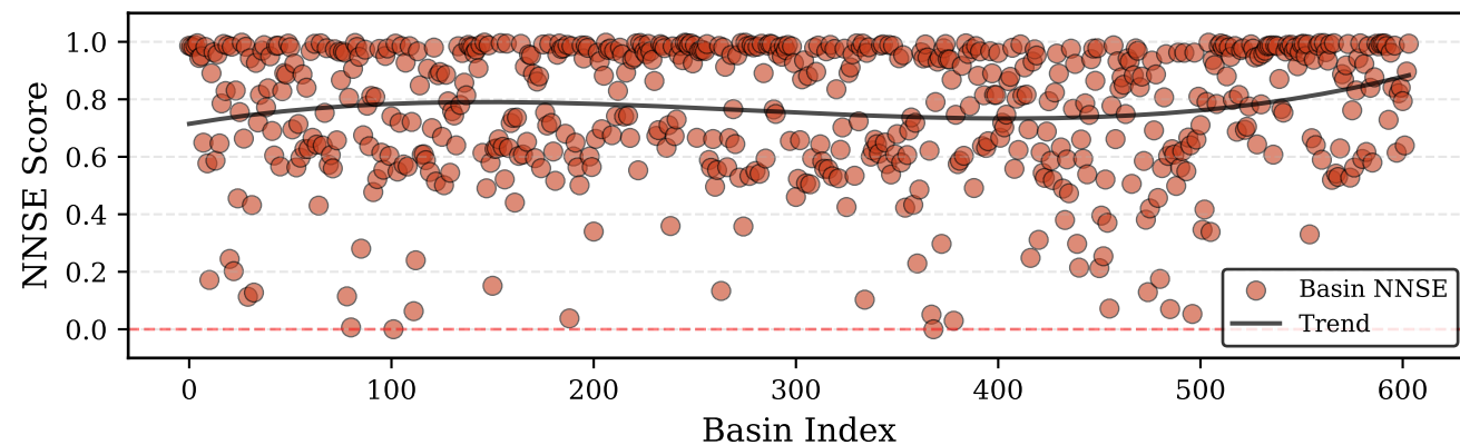
LSTM
