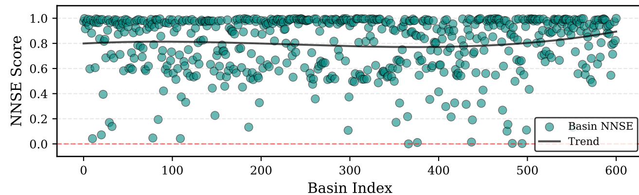
Informer
