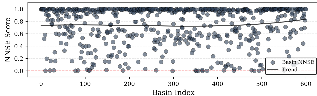
FEDformer
