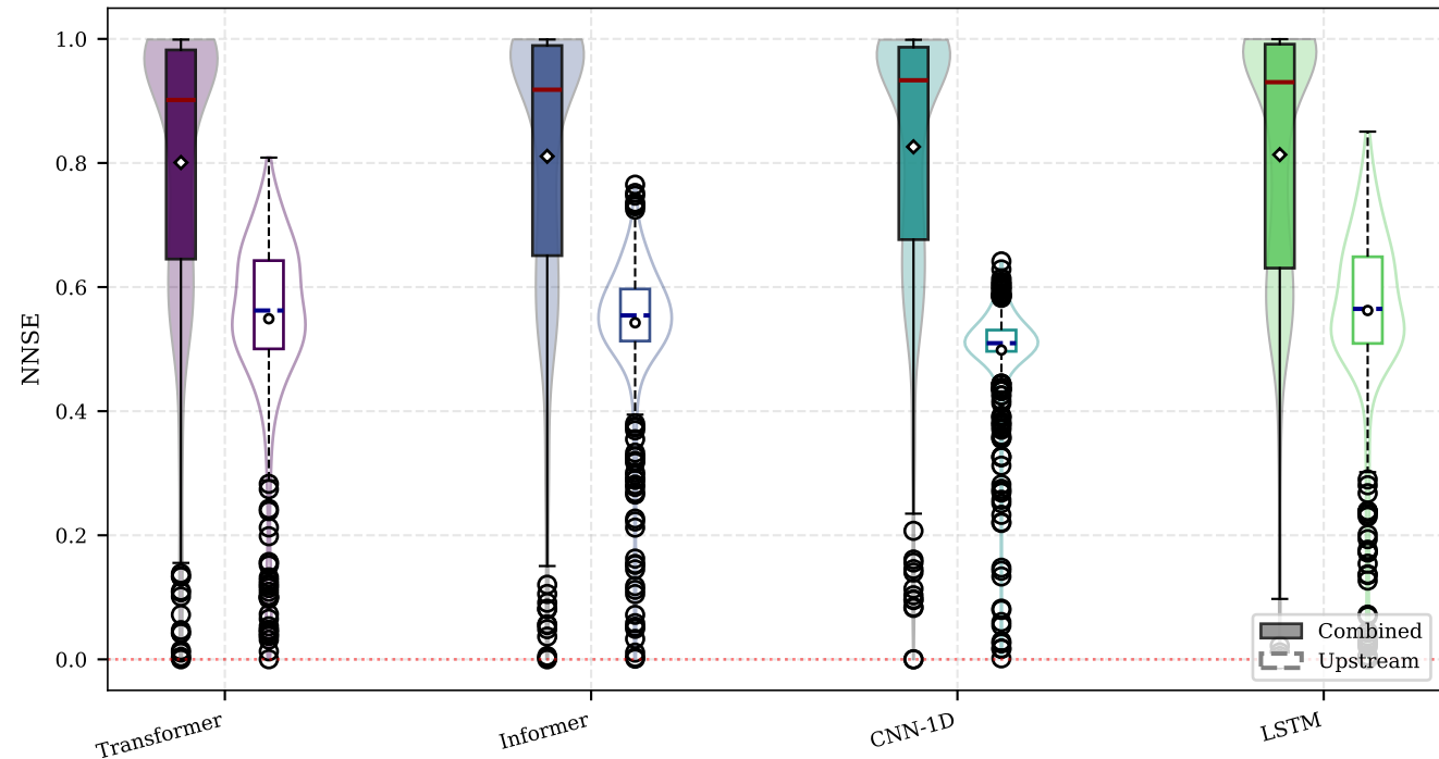
Distribution Comparison: Combined vs Upstream (Violin + Box Plot)
