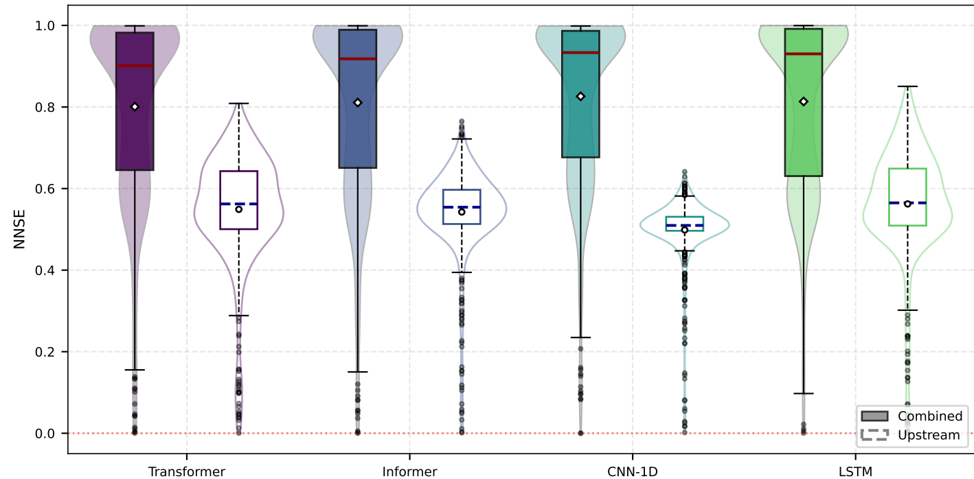
Distribution Comparison: Combined vs Upstream
