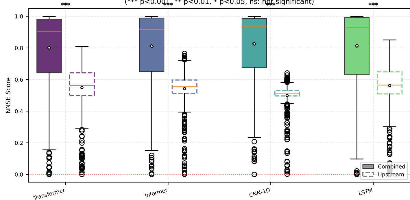
Model Performance Comparison: Combined vs Upstream (*** p < 0.001 , ** p < 0.01 , * p < 0.05 , ns: not significant)
