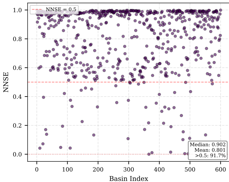
CNN-1D
