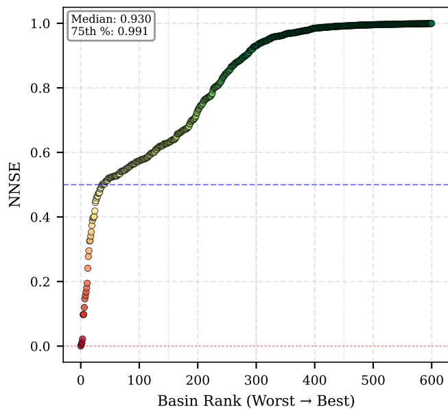
LSTM
