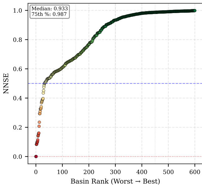
CNN-1D
