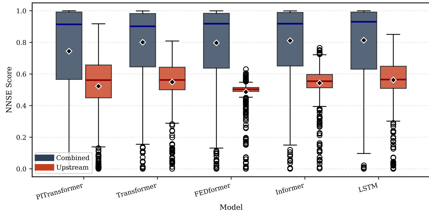
NNSE Distribution: Combined vs Upstream Inputs
