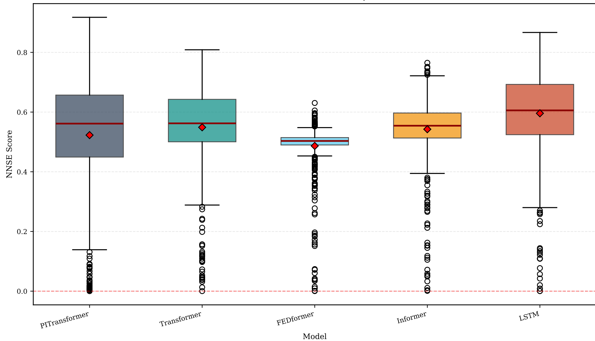
Distribution of NNSE Scores by Model
