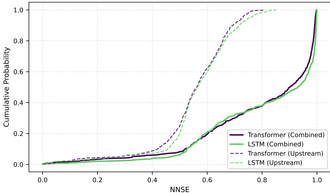
CDF of NNSE Scores
