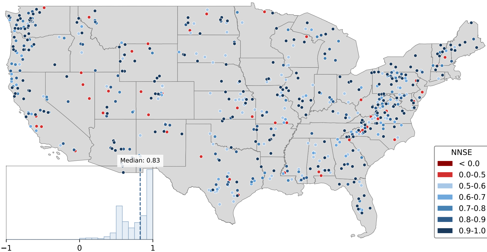
(a) Spatial Distribution of NNSE for Combined Configuration
