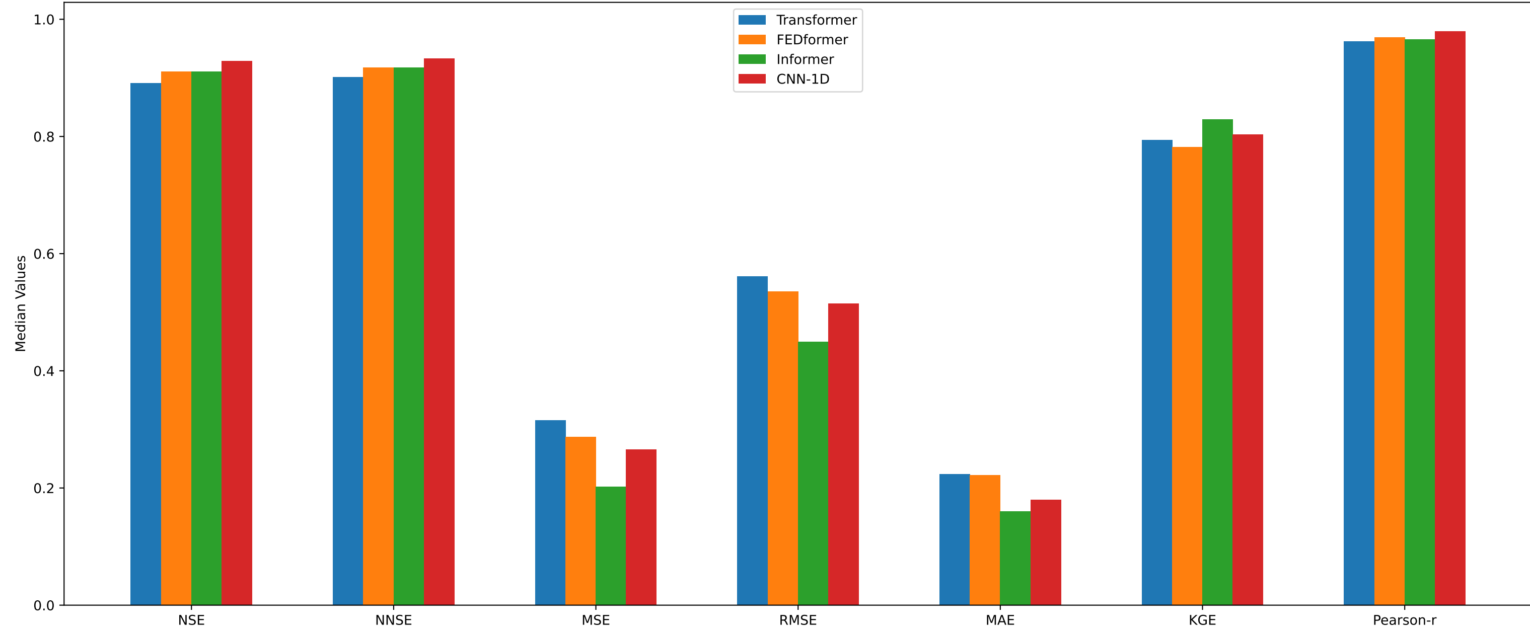
Median Performance Comparison Across Models (Combined Dataset)
