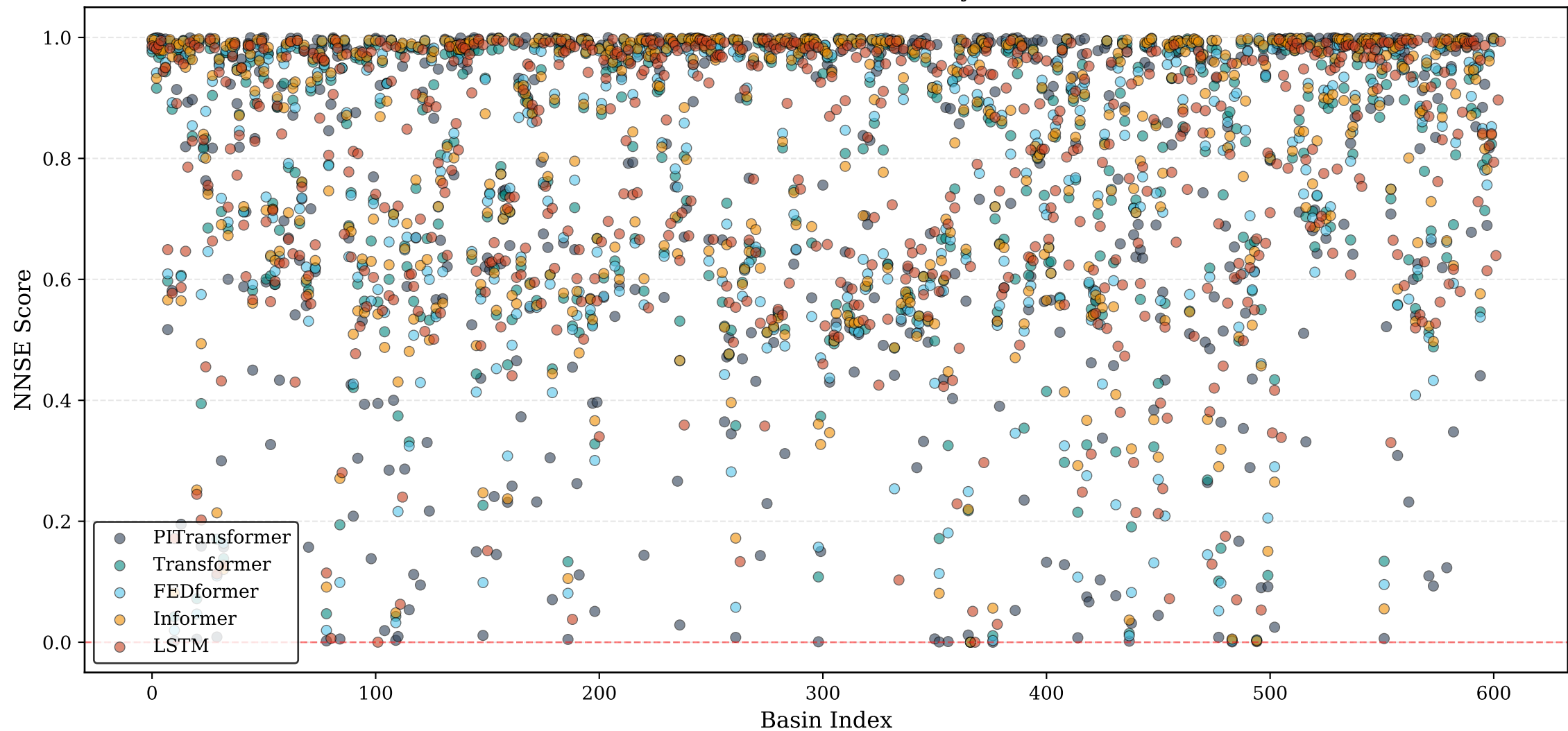
NNSE Scores Across Basins by Model
