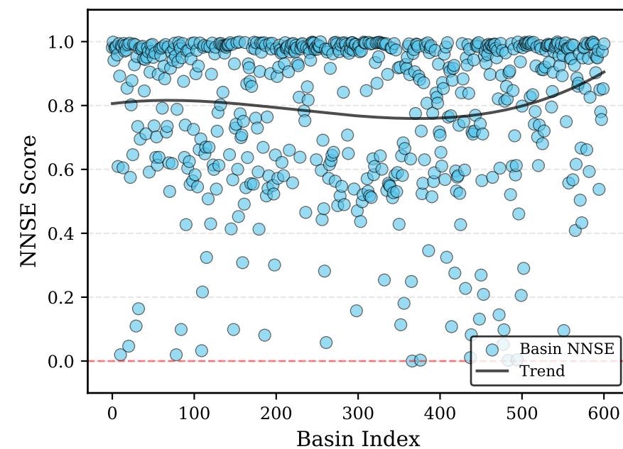
FEDformer
