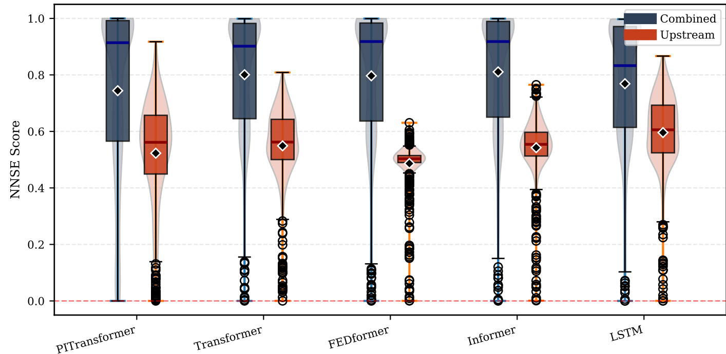
NNSE Distribution by Model: Combined vs Upstream
