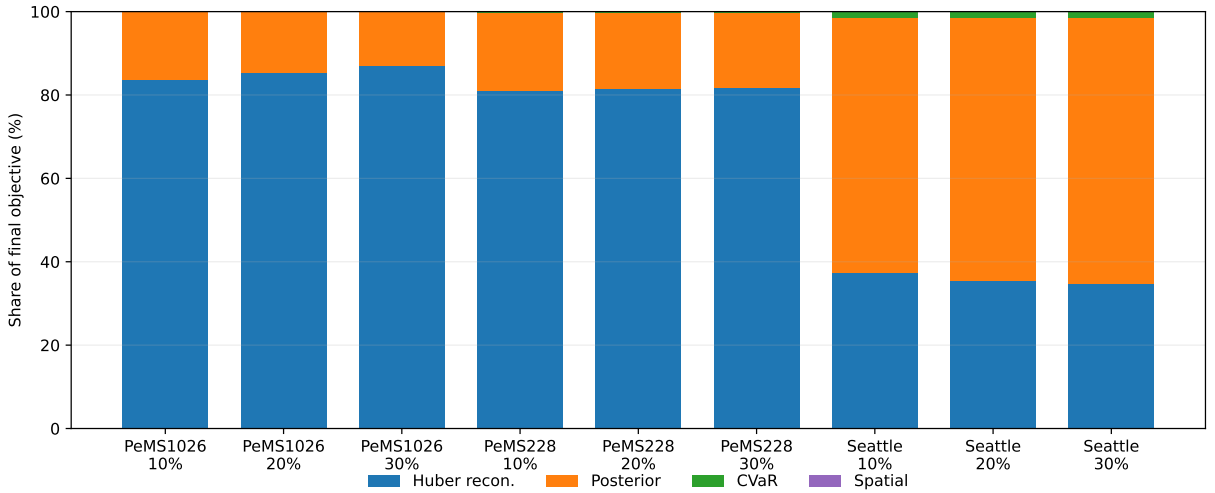
Figure A.8: Current-best TRACE-BiOpt final-objective composition. Each bar shows the mean weighted share of the accepted final objective coming from hidden Huber reconstruction loss, posterior trace, scenario-CVaR trace, and spatial regularization over the ten split-specific runs of that row.
