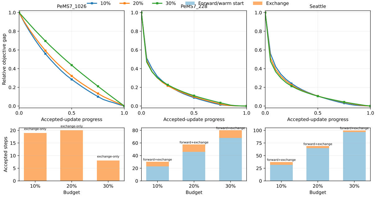
Figure 4: Current-best TRACE-BiOpt objective descent and accepted-step mix. The top row shows the mean relative objective gap remaining over normalized accepted-update progress; the bottom row stacks the mean accepted forward/warm-start and exchange steps for each budget.
