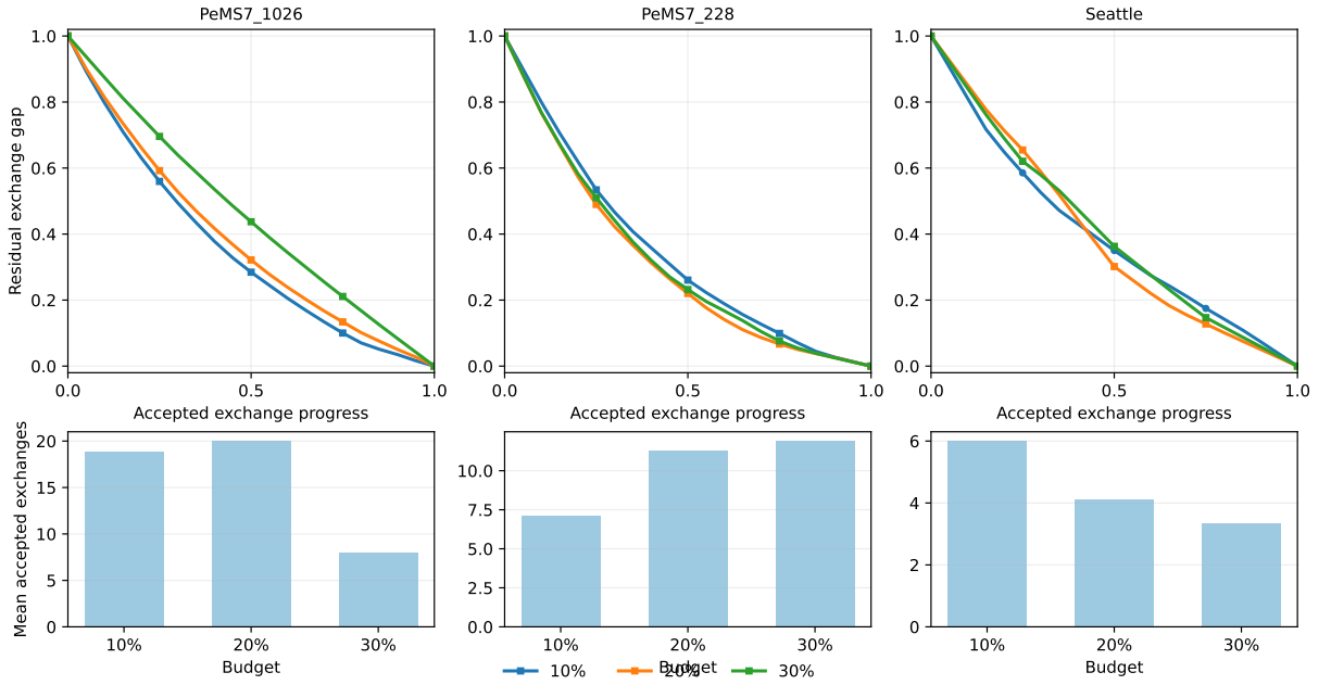
Figure A.7: Current-best TRACE-BiOpt residual exchange-gap profiles. The top row shows the mean fraction of eventual exchange-phase improvement still remaining after the accepted exchange phase begins; the bottom row reports the mean number of accepted exchange steps, with '0-ex' annotations giving how many of the ten split-specific runs accepted no exchange at all beyond the forward or warm-start layout.
