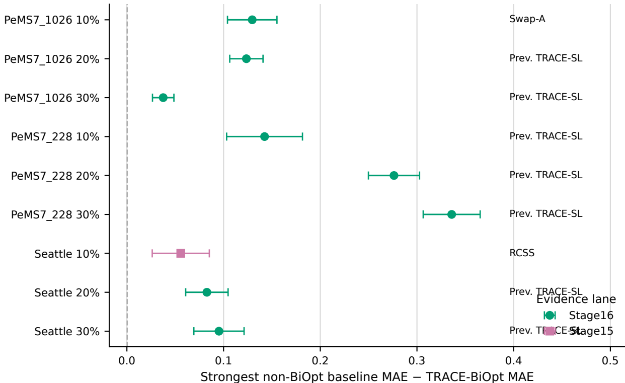
Paired current-best dominance margins across tested regimes
