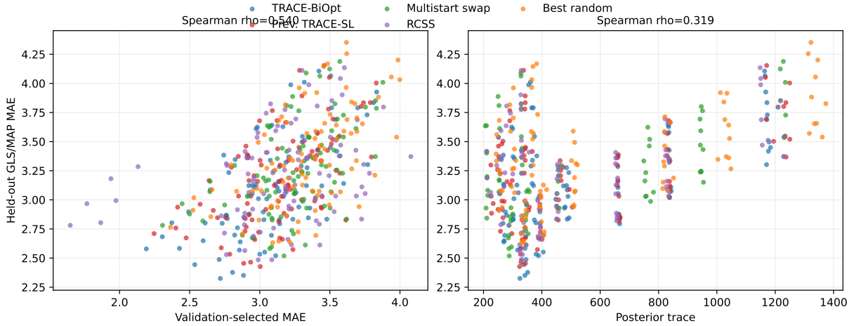
Figure 6: Mechanism-alignment diagnostics on the 450 GLS/MAP selected-layout rows formed by three networks, three budgets, ten seeds, and five layout families. Left: validation-selected MAE versus held-out MAE. Right: posterior trace versus held-out MAE on the same selected layouts.
