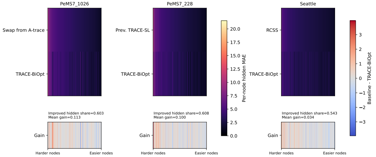
Figure 9: Representative low-budget common-hidden error heatmaps on the seed-25 current-best rows. Within each dataset, columns are the nodes that remain hidden under both layouts, ordered from higher to lower strongest-baseline hidden-node MAE. The top heatmap compares node-wise hidden MAE for the strongest baseline and TRACE-BiOpt; the bottom strip shows baseline minus TRACE-BiOpt, so positive values favor TRACE-BiOpt.
