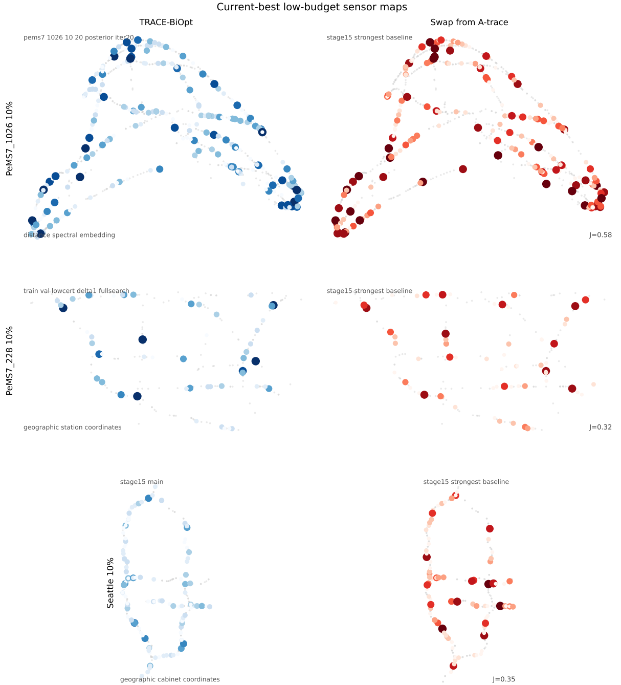
Figure 7: Current-best low-budget sensor maps. PeMS7_228 and Seattle use released geographic sensor coordinates; PeMS7_1026 uses a distance-derived network embedding because benchmark station coordinates are not released with the public artifact. Darker and larger markers indicate nodes selected in more of the ten split-specific layouts.
