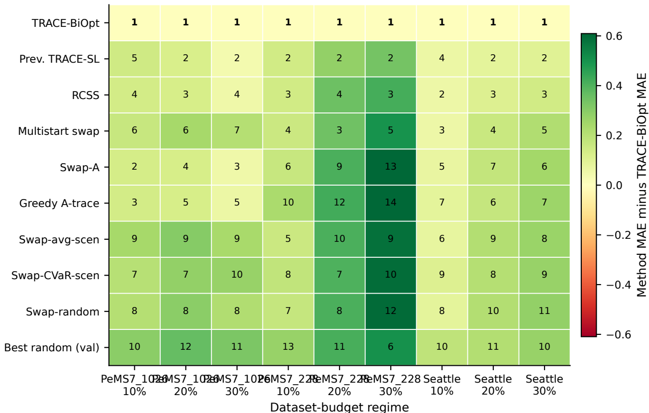
Compact baseline matrix: TRACE-BiOpt plus top 9 challengers
