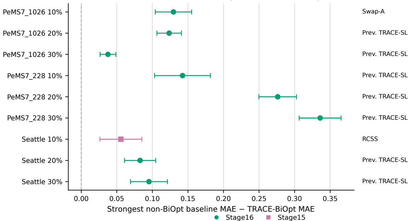
Paired current-best dominance margins across tested regimes
