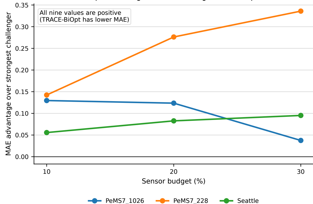
TRACE-BiOpt advantage over the strongest non-BiOpt baseline
