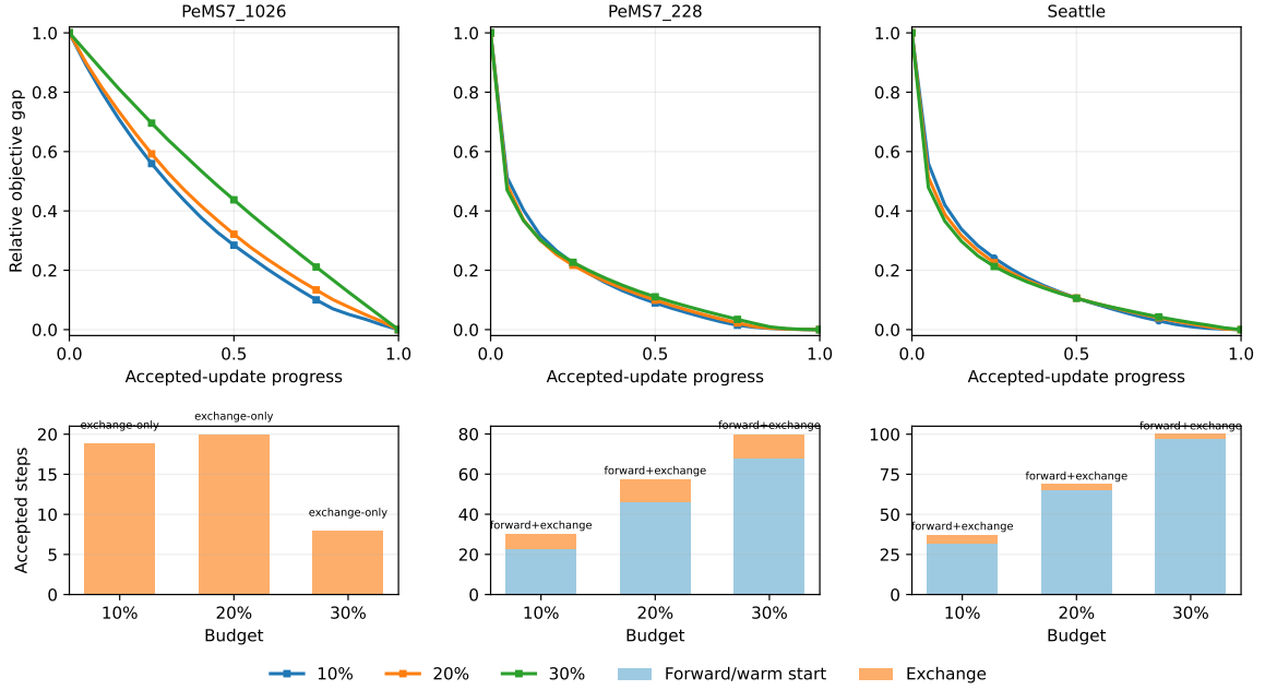
Figure 4: Current-best TRACE-BiOpt objective descent and accepted-step mix. The top row shows the mean relative objective gap remaining over normalized accepted-update progress; the bottom row stacks the mean accepted forward/warm-start and exchange steps for each budget.
