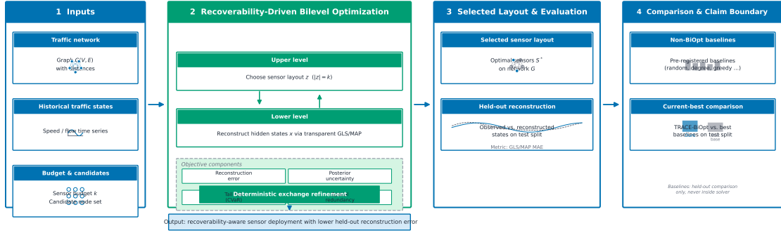
Figure 1: TRACE-BiOpt framework. The method optimizes a single recoverability-driven bilevel sensor-layout objective: a transparent GLS/MAP lower-level reconstruction is embedded inside an upper-level hidden-state risk objective with posterior-uncertainty, tail-risk, and spatial-redundancy terms. Baselines are used only for held-out evaluation and do not enter the solver.
