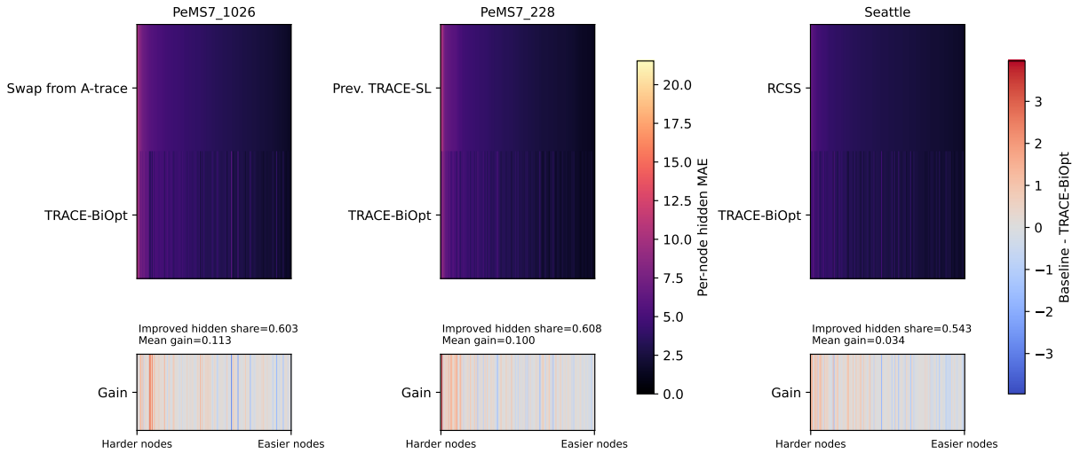
Figure A.4: Representative low-budget common-hidden error heatmaps on the seed-25 current-best rows. Within each dataset, columns are the nodes that remain hidden under both layouts, ordered from higher to lower strongest-baseline hidden-node MAE. The top heatmap compares node-wise hidden MAE for the strongest baseline and TRACE-BiOpt; the bottom strip shows baseline minus TRACE-BiOpt, so positive values favor TRACE-BiOpt.
