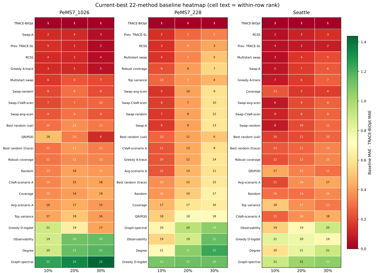
Figure 12: Current-best 22-method baseline heatmap. Each panel corresponds to one dataset; columns are sensor budgets, cell color is baseline MAE minus TRACE-BiOpt MAE, and the number inside each cell is the within-row rank. Nonnegative cells therefore indicate that the corresponding baseline does not beat TRACE-BiOpt on that dataset-budget row. The highlighted TRACE-BiOpt row stays rank 1 in all nine cells.
