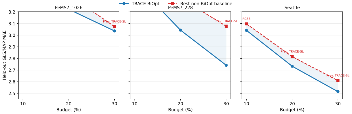
Figure 3: Strongest-challenger envelope across sensor budgets. Each panel plots TRACE-BiOpt against the row-specific strongest pre-registered non-BiOpt baseline from the current-best evidence chain. The strongest challenger may differ across budgets. TRACE-BiOpt remains the lower-MAE curve on every dataset-budget row.
