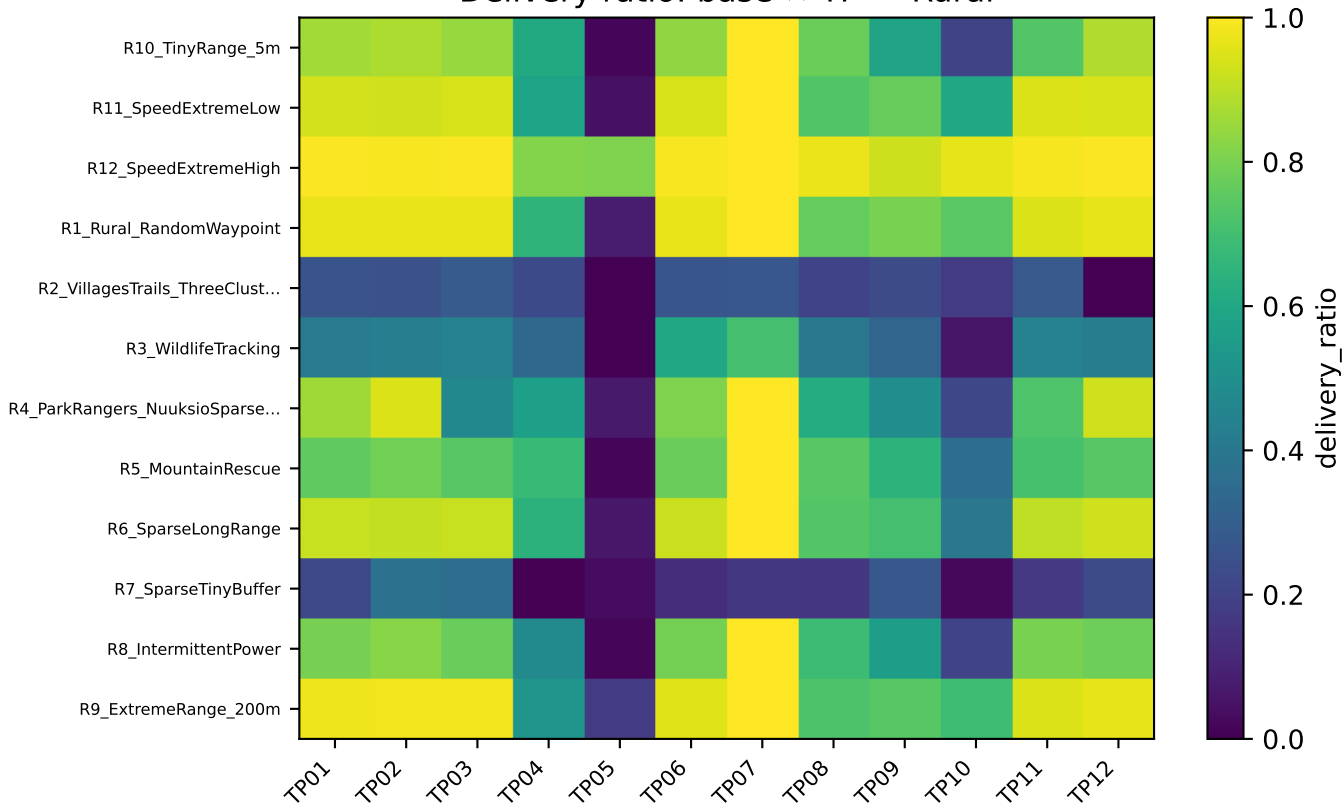
Delivery ratio: base × TP — Rural
