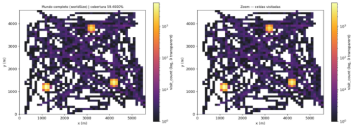
TP08
