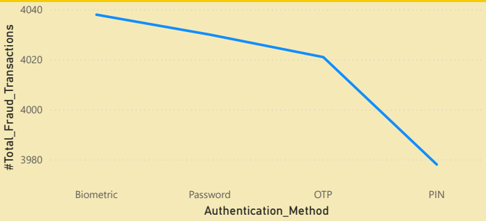
Fraud by Authentication Method
