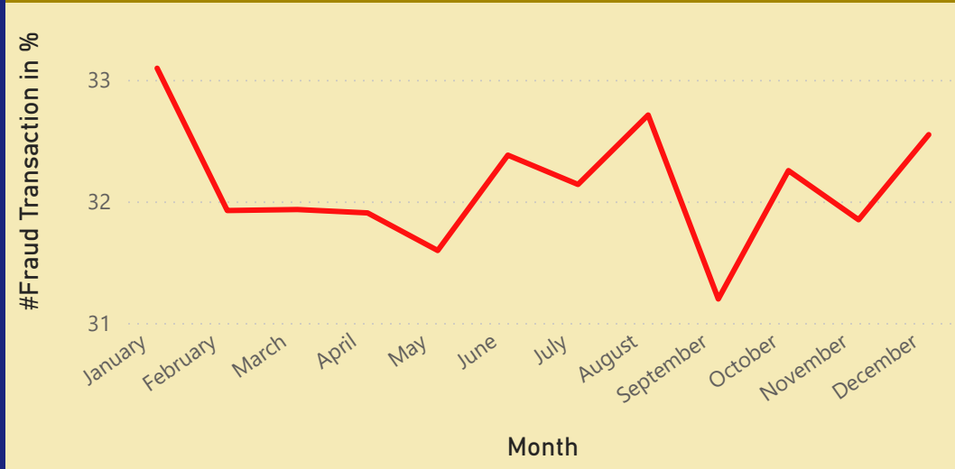
Fraud Trend Over Time
