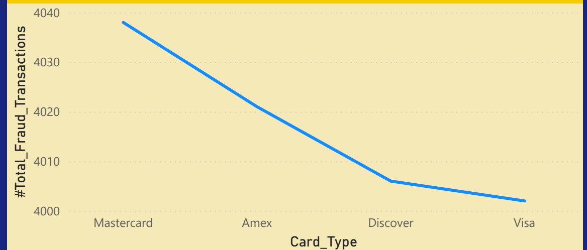
Card type wise Fraud transaction count
