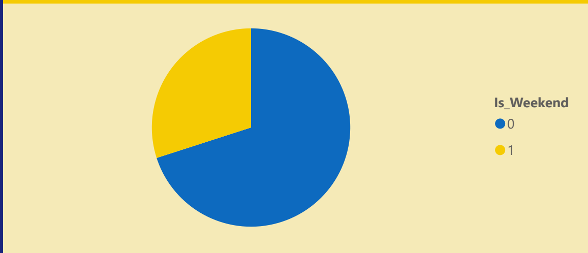
Weekend Vs Fraud Count
