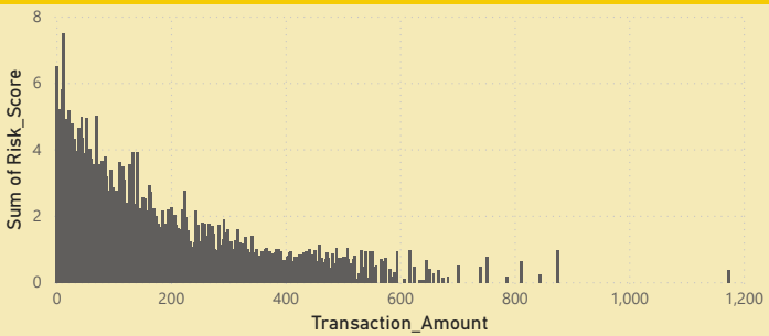
Transaction Amount vs Risk Score
