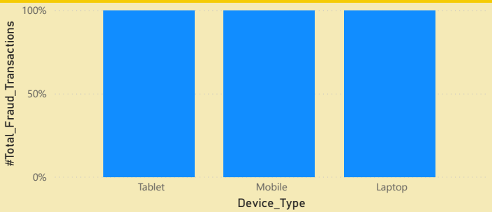
Fraud by Device Type
