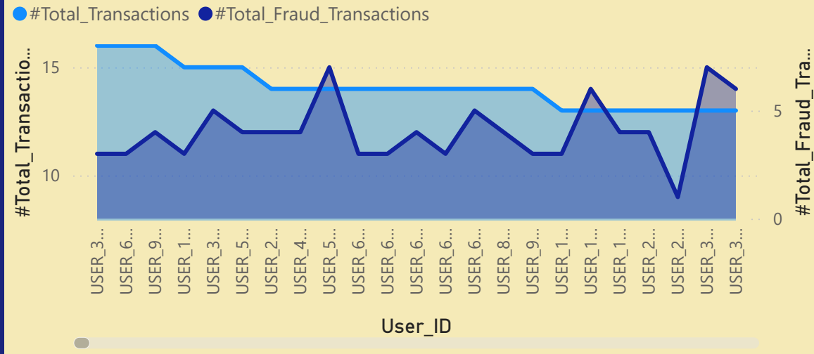
Total Transactions Vs Fraud Transactions
