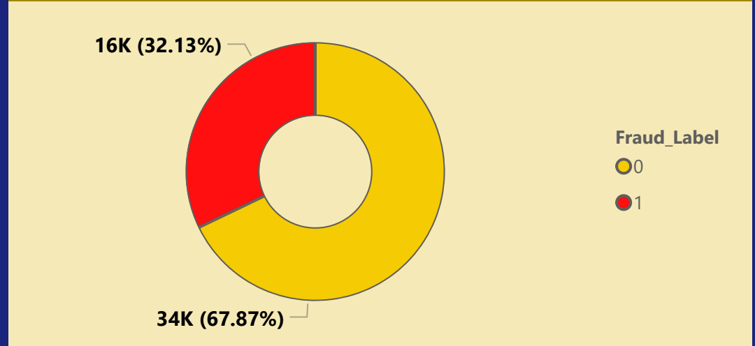
Fraud vs Non-Fraud Comparison
