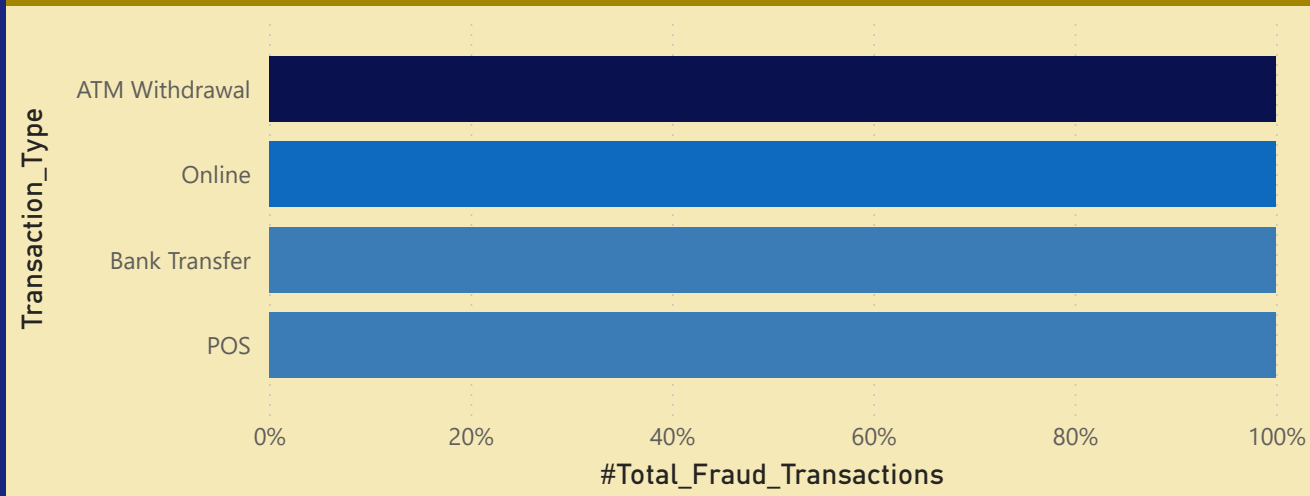
Fraud by Transaction Type
