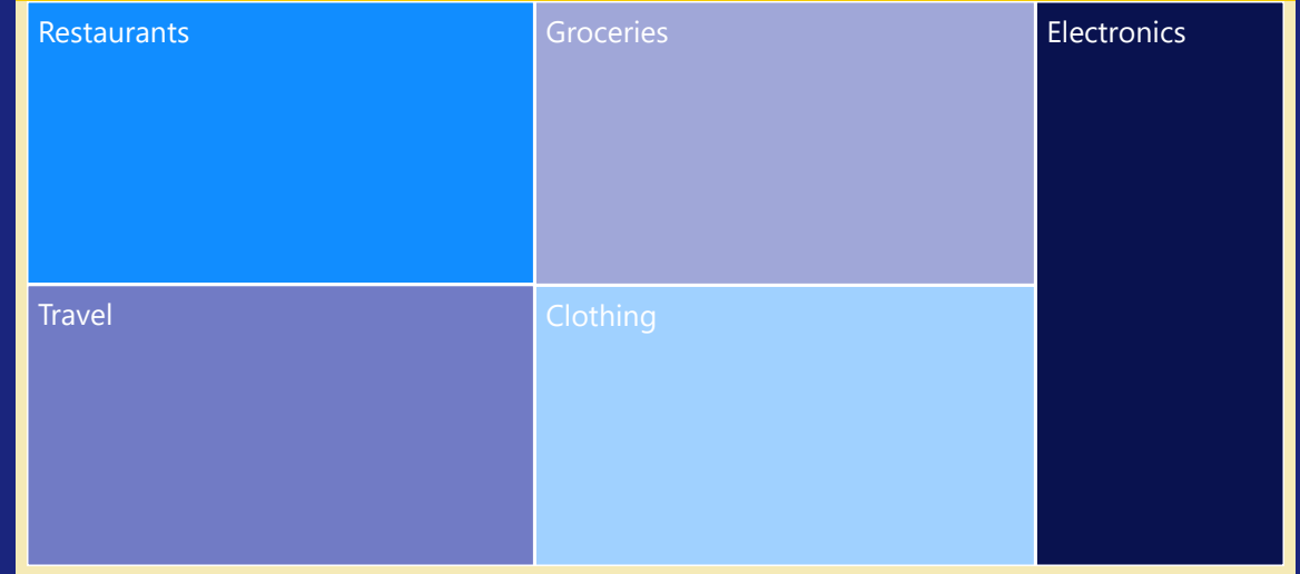
Marchant Category wise Fraud Count
