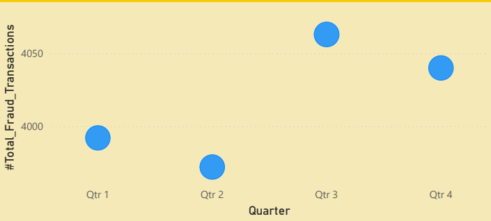
Quarterly Fraud Analysis
