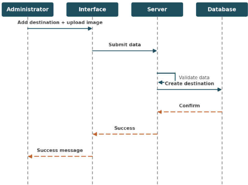
Figure 5.7 — Sequence diagram: Administrator Adds a Destination
