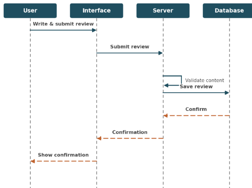
Figure 5.6 — Sequence diagram: Submit Review
