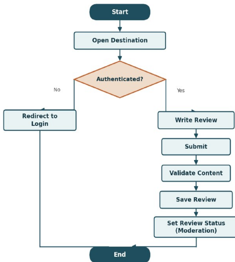
Figure 6.4 — Activity diagram: Submit Review
