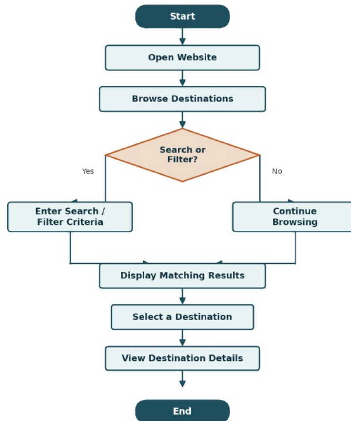
Figure 6.1 — Activity diagram: Browse / Search Destination
