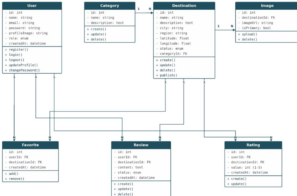
Figure 4.1 — Class diagram of Morocco Explore
