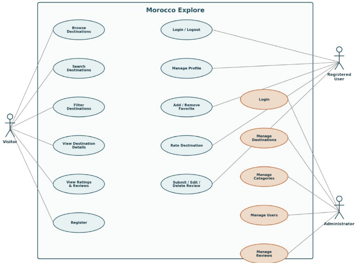
Figure 2.1 — Use case diagram of Morocco Explore
