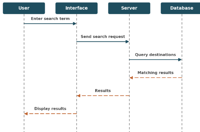
Figure 5.3 — Sequence diagram: Search Destination
