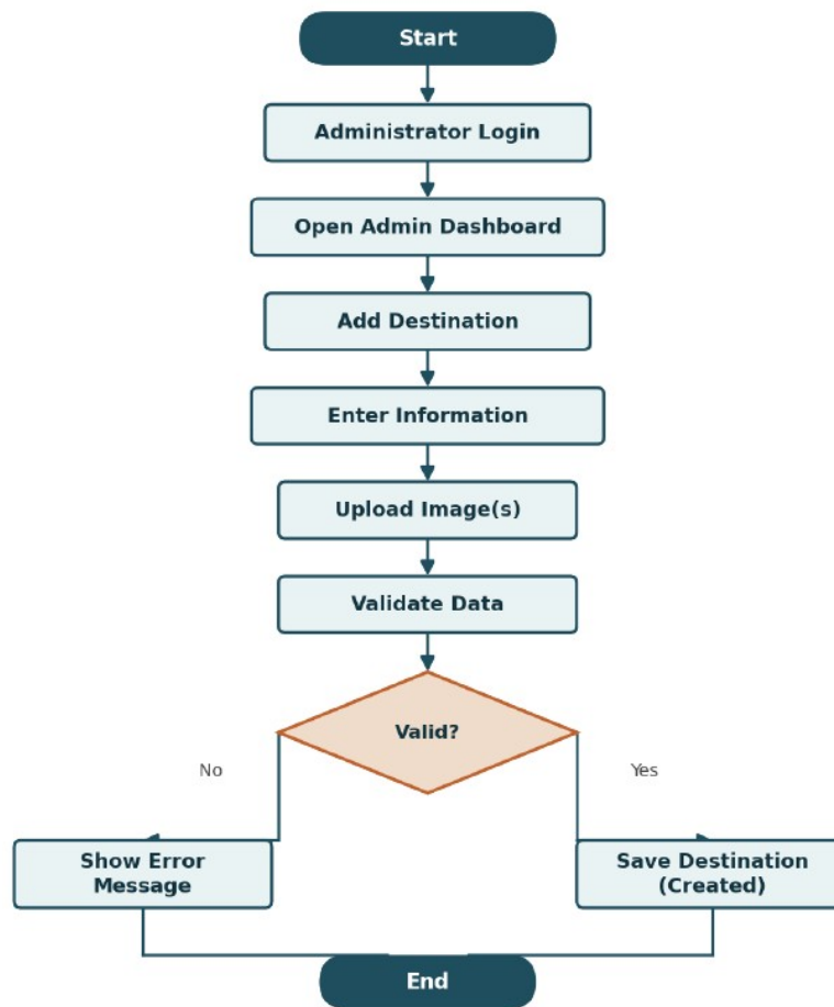
Figure 6.5 — Activity diagram: Administrator Adds a Destination
