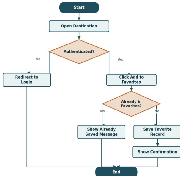
Figure 6.3 — Activity diagram: Add Favorite
