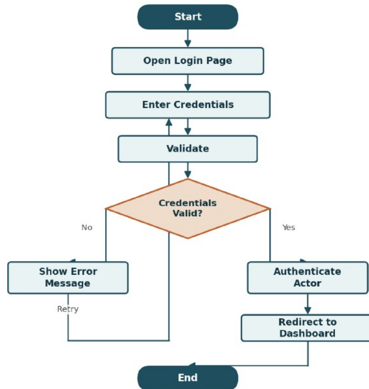
Figure 6.2 — Activity diagram: User Login
