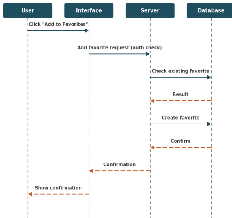
Figure 5.5 — Sequence diagram: Add Favorite
