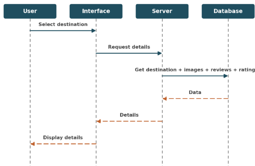
Figure 5.4 — Sequence diagram: View Destination Details
