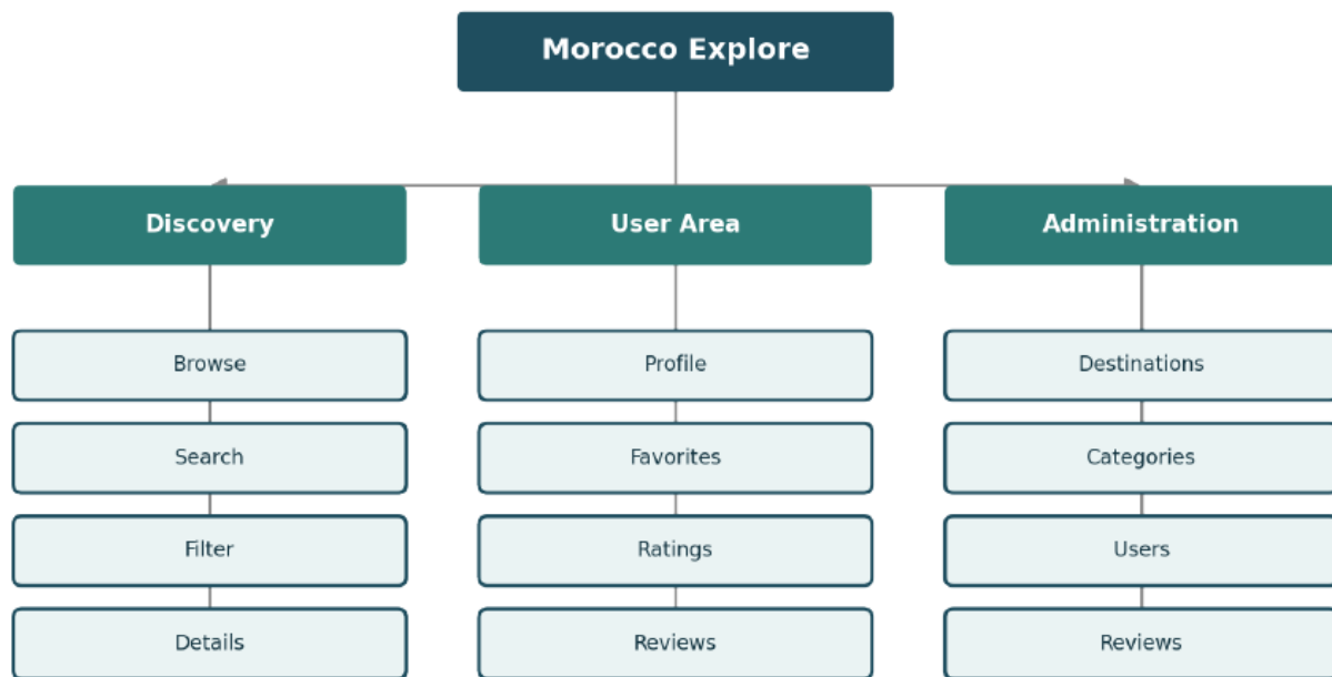
Figure 1.1 — Functional overview of Morocco Explore
