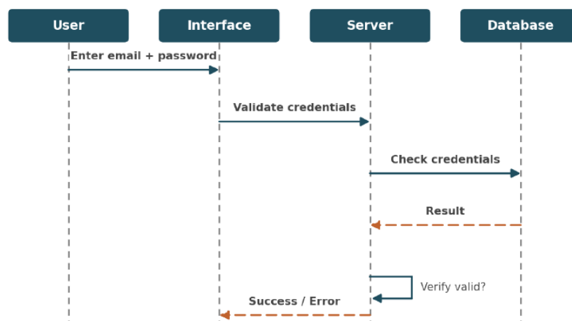
Figure 5.2 — Sequence diagram: User Login
