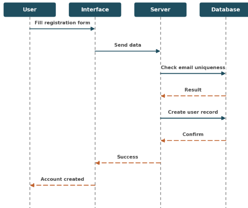
Figure 5.1 — Sequence diagram: User Registration
