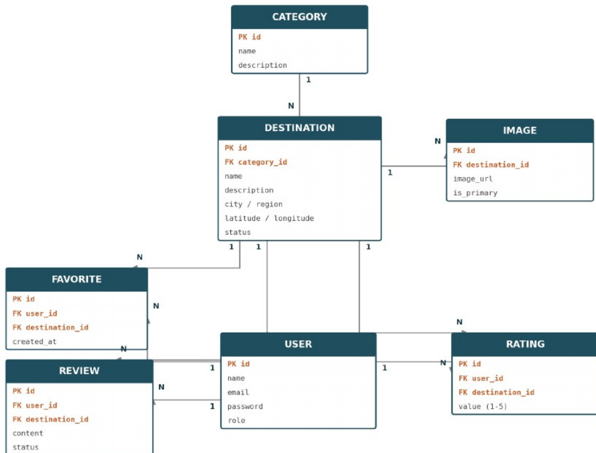
Figure 7.1 — Entity-Relationship Diagram (ERD)
