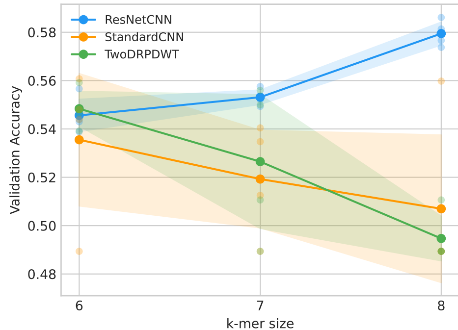
Accuracy vs k-mer size
