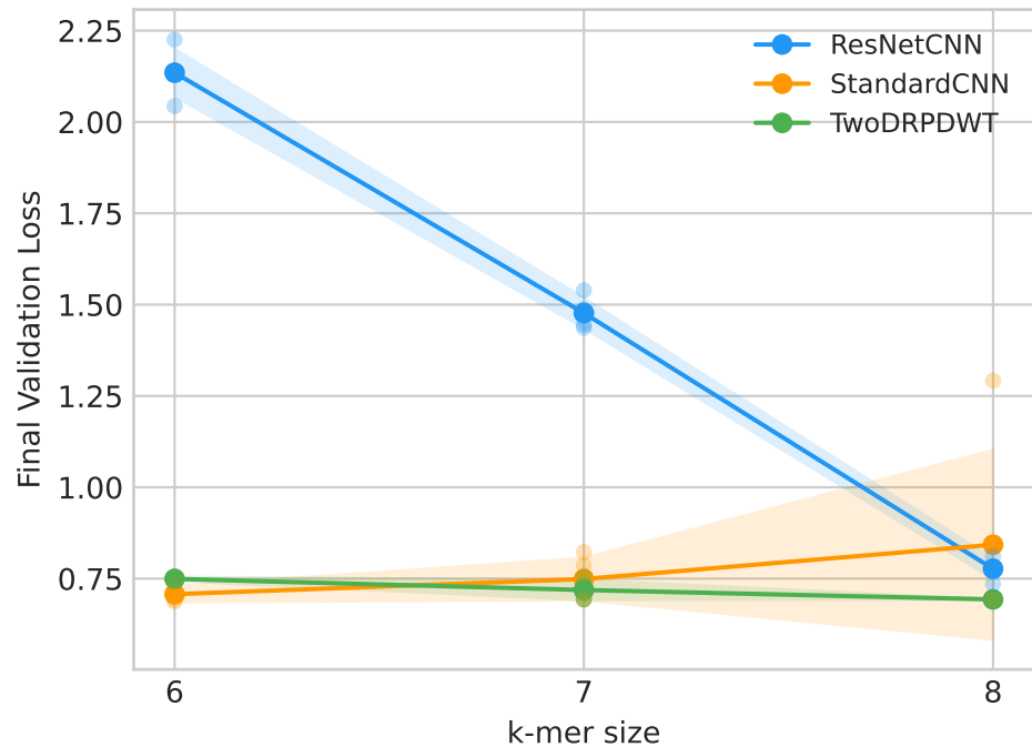
Validation Loss vs k-mer size
