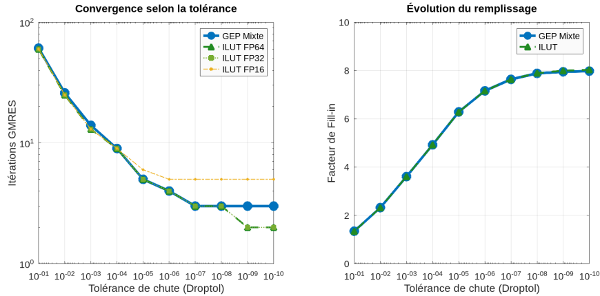
Figure 4: GMRES iteration count (left) and Preconditioner fill-in factor (right) as a function of the drop tolerance (Phase 2, 494_bus).
