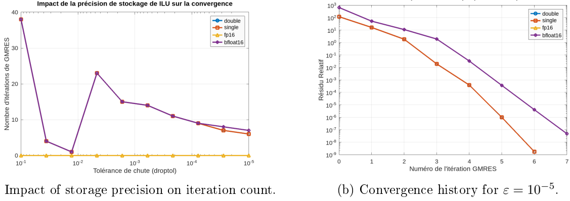
Figure 3: Exploratory uniform multi-precision simulation results on the bcsstk08 matrix.
