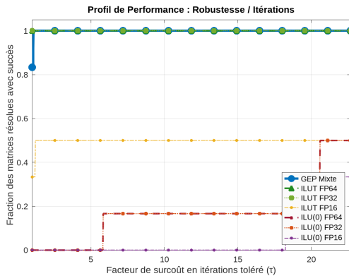
(a) Iteration profile (including ILU(0)).
