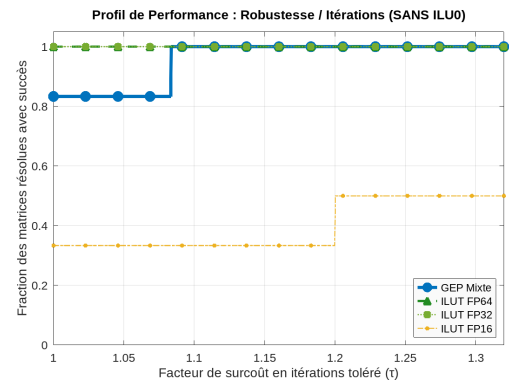
(b) Iteration profile (excluding ILU(0)).
