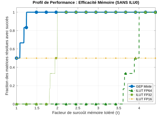
(b) Memory profile (excluding ILU(0)).
