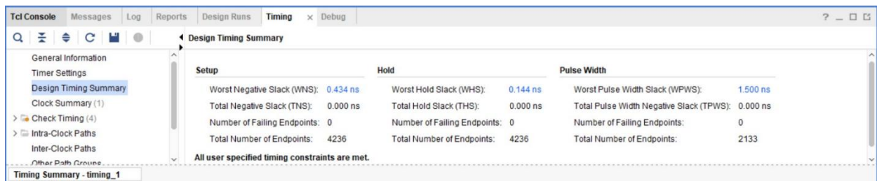
Timing analysis Pre-PnR (fitting)
