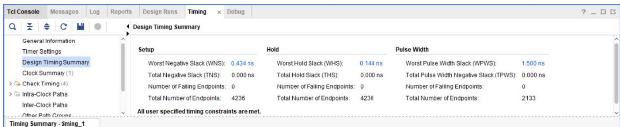
Figure 14 Timing analysis Pre-PnR (fitting)
