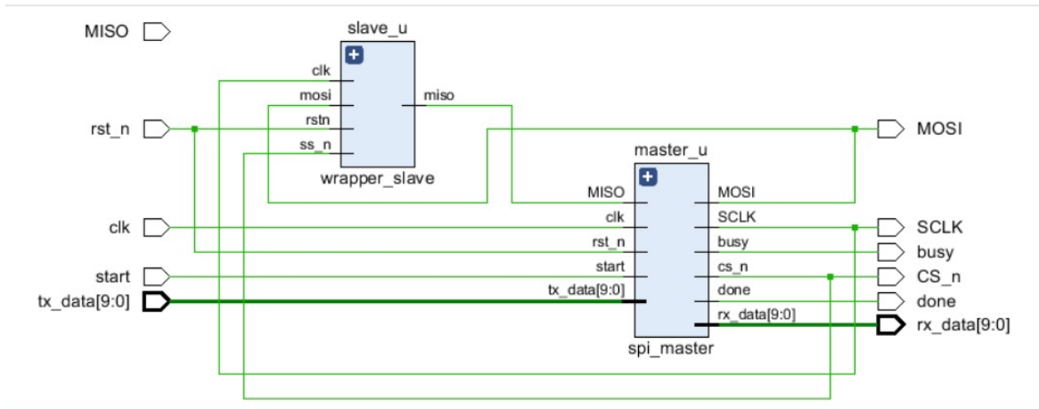
Figure 20 Block diagram of Integration SPI master/slave
