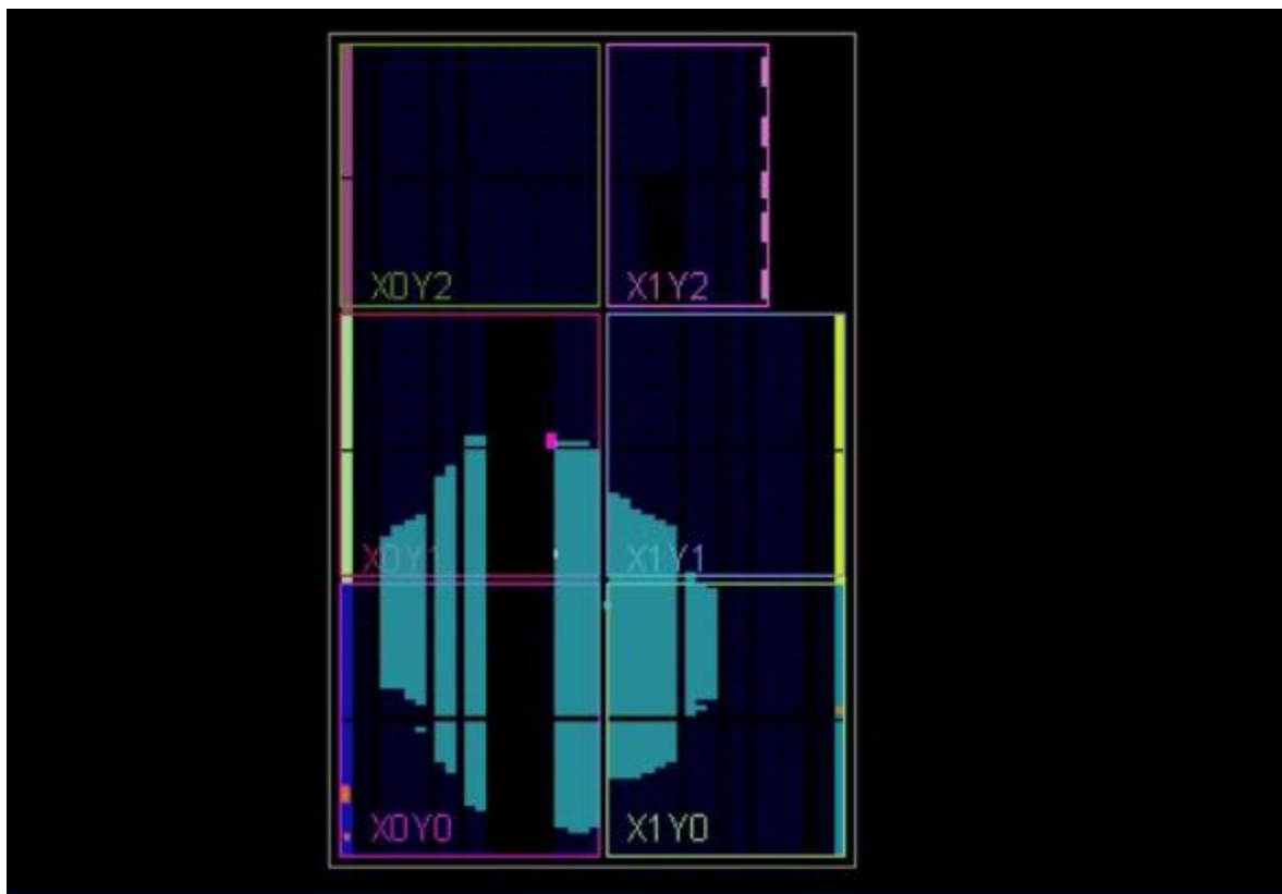
Figure 16 Schematic & Routing of slave and RAM
