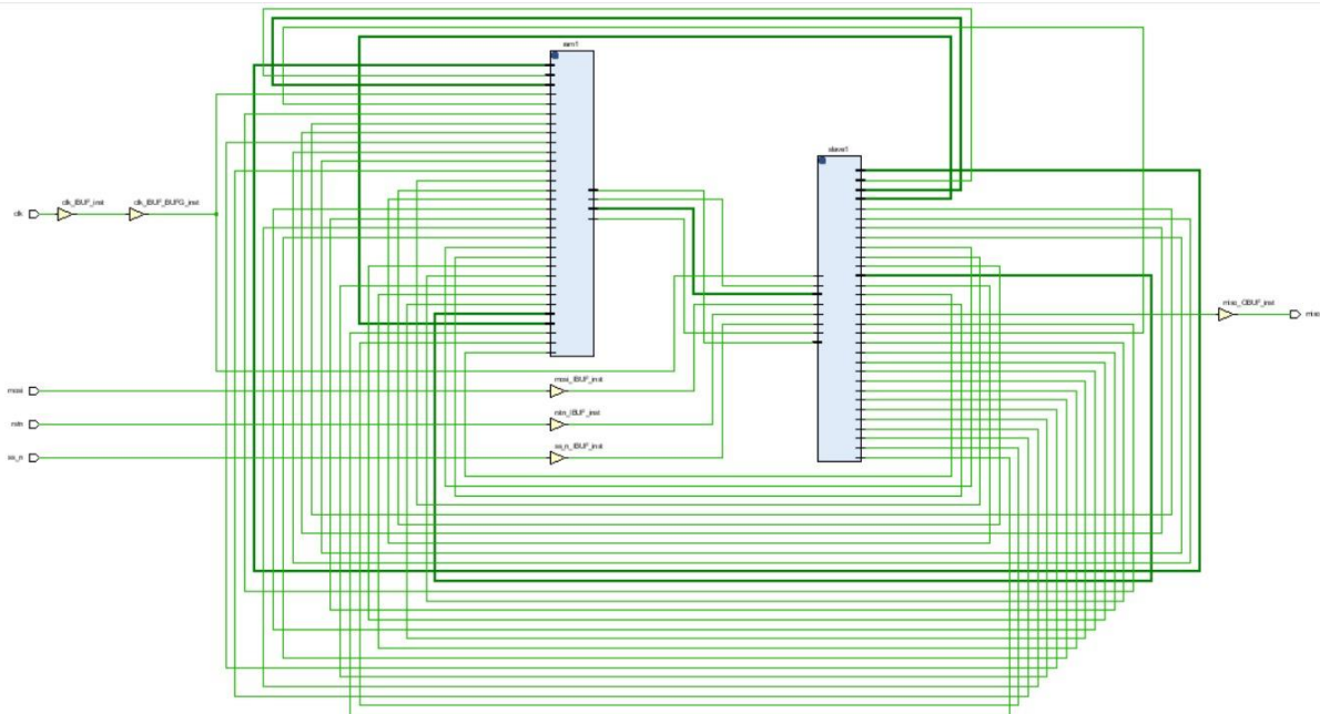
Figure 16 Schematic & Routing of slave and RAM
