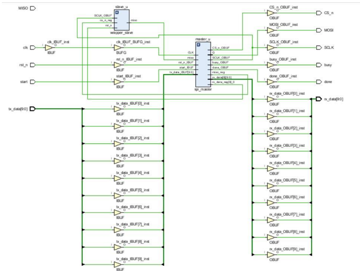
Figure 21 Schematic & routing of SPI Master/Slave
