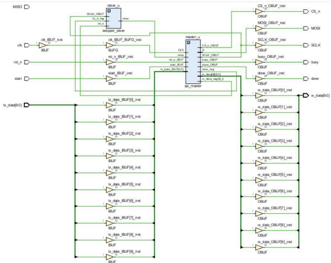
Figure 21 Schematic & routing of SPI Master/Slave
