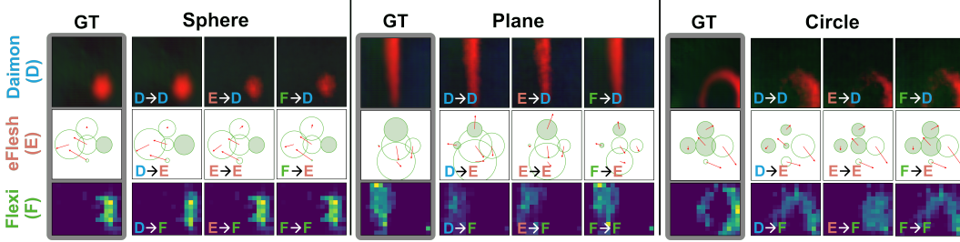
Figure 5: Self- and cross-reconstruction from the shared latent. We visualize representative validation contacts from sphere, plane, and circle indentors. For each sensor, the first column is the ground-truth observation, the diagonal entries are self-reconstructions, and the off-diagonal entries are cross-reconstructions decoded from the nearest latent representations of the other sensors in the validation set.
