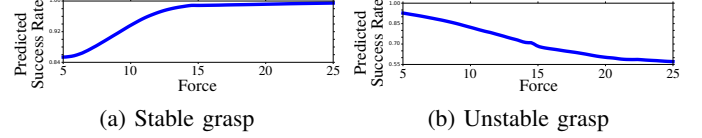
Figure 4: Predicted grasp success rate with varying the amount of force F . The model learned that, when stably in contact with the object, there is a correlation between force applied and success rate . However, for unstable grasps, the model learned that increasing the grasp force might misplace the object and result in an unsuccessful grasp.
