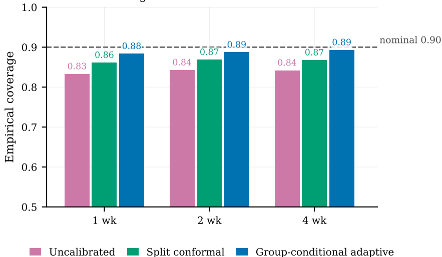
Interval coverage before and after calibration
