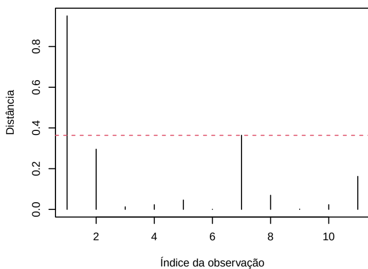
Cook's distance
