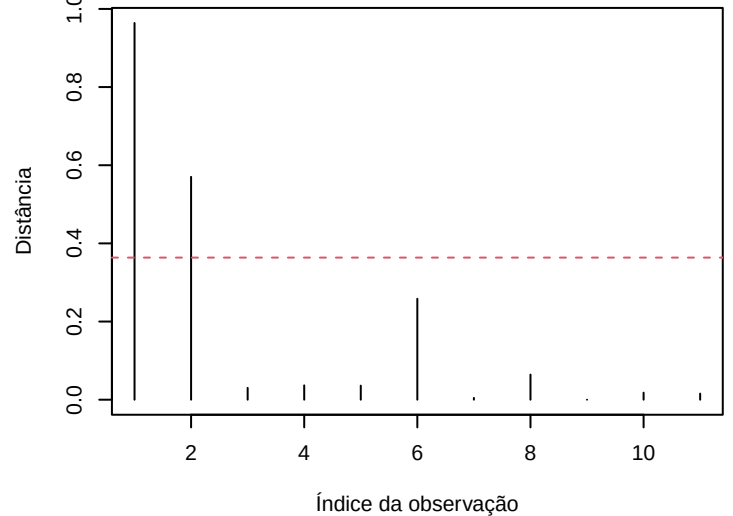
Cook's distance
