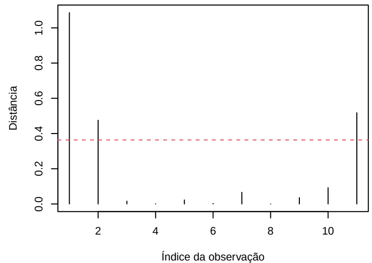
Cook's distance
