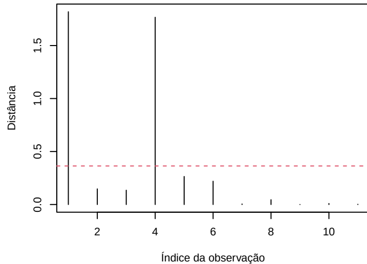
Cook's distance
