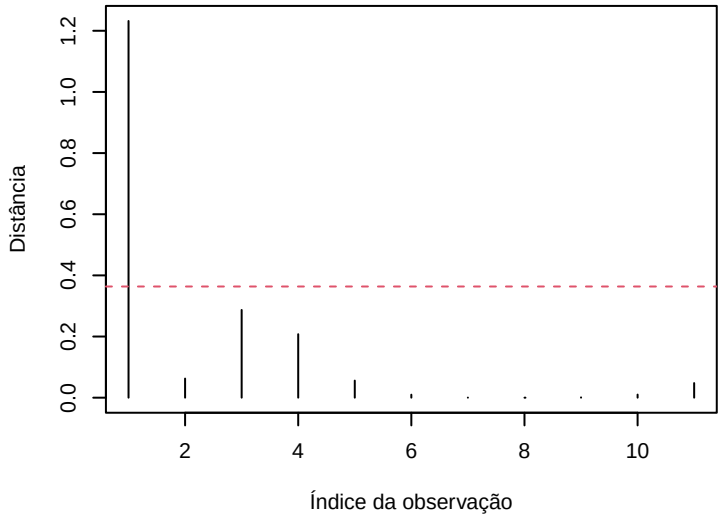
Cook's distance
