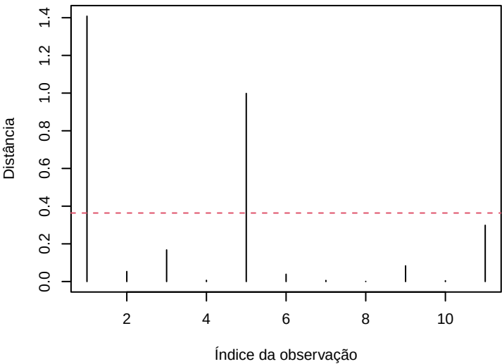
Cook's distance
