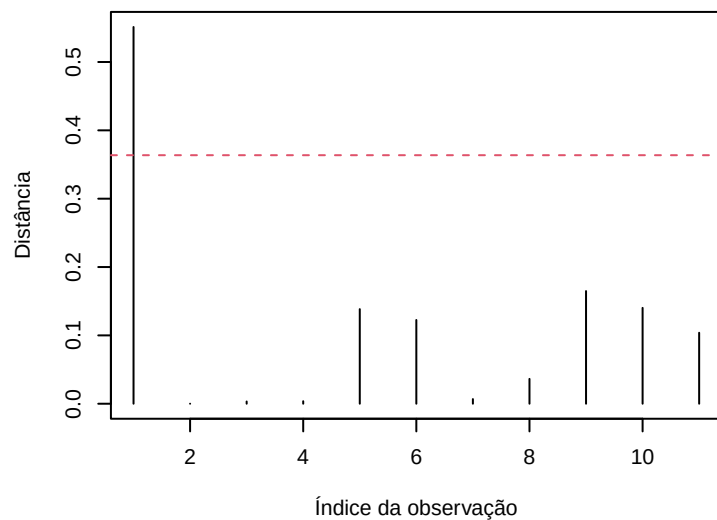
Cook's distance
