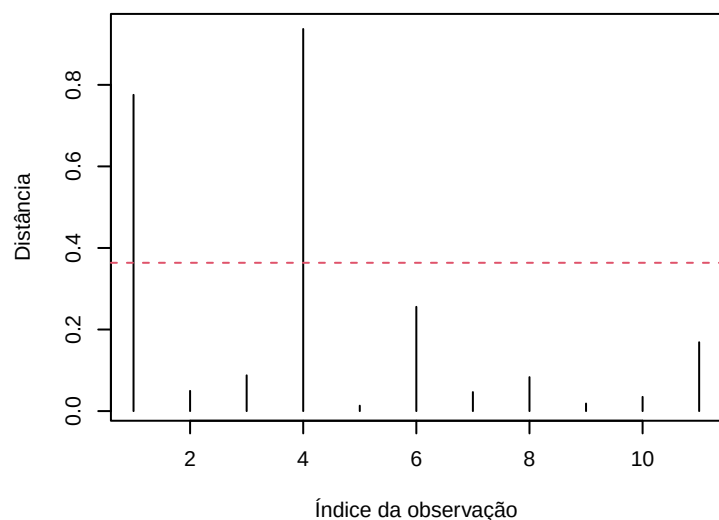
Cook's distance
