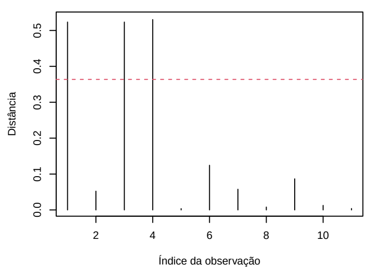
Cook's distance
